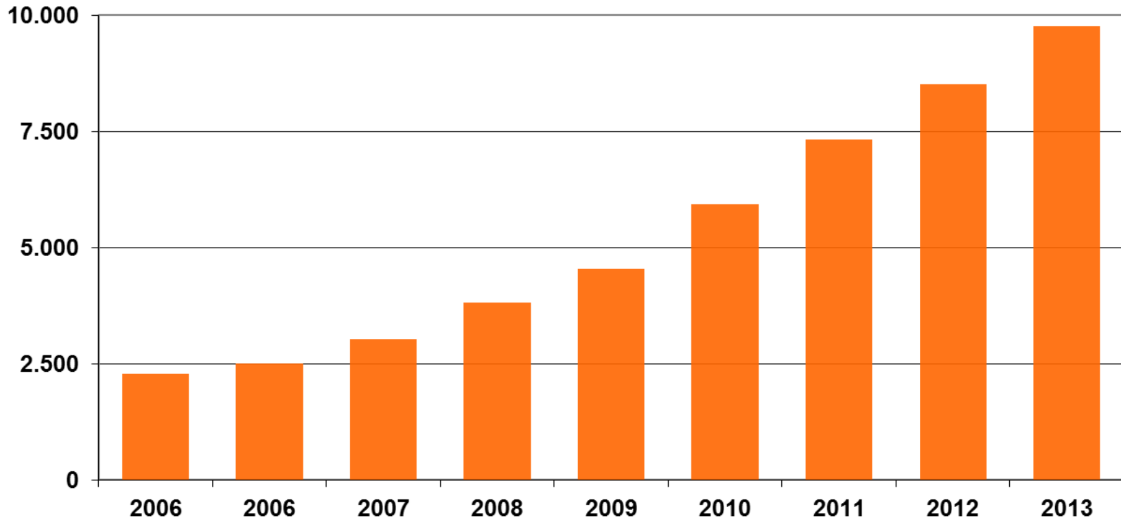
Directory of Open Access Journals: Number of Journals per year
